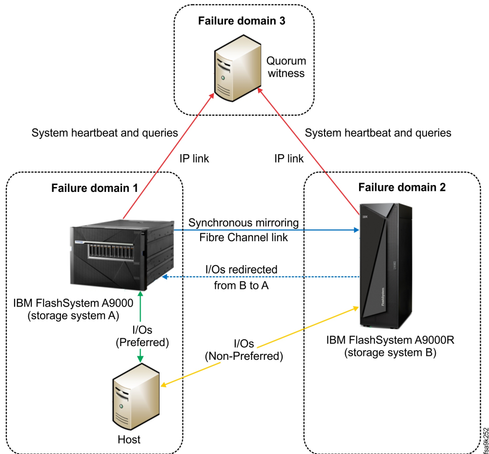
Figure 1. Typical HyperSwap solution with the Quorum Witness
